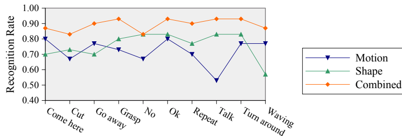
Fig. 3: Evaluation of FINGeR on a set of 10 dynamic gestures.
