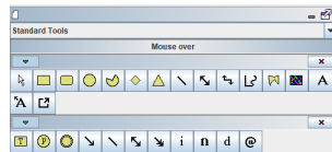
Figure 4.2: The Petri Net Toolbars in the Renew main Window
