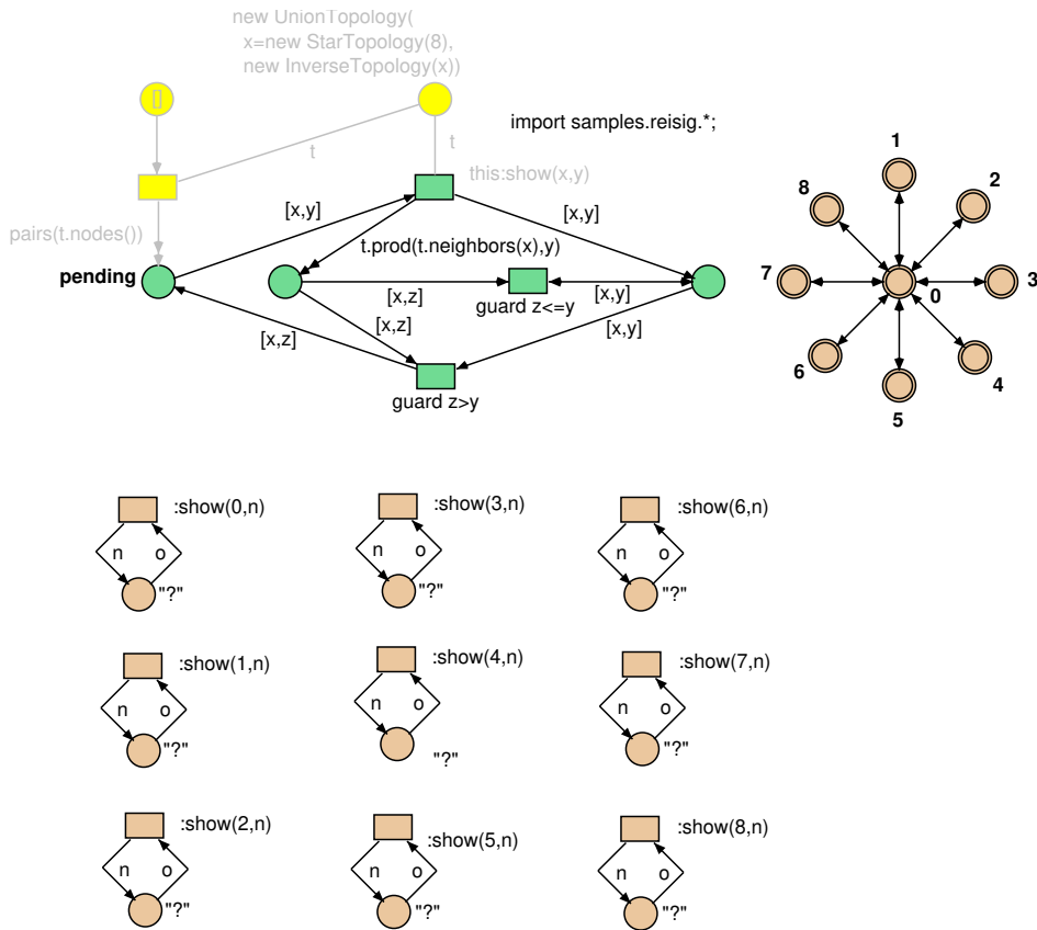
Figure 3.26: The net visualelection
