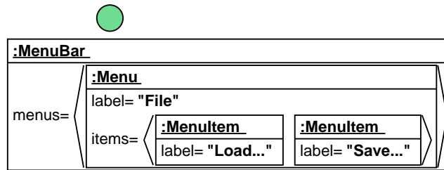
Figure 4.4: An Example of Browsing Token Objects in Expanded Tokens Mode
