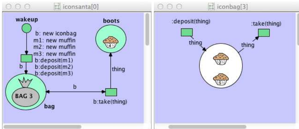
Figure 4.7: The Santa Claus Example with Icons During Simulation.
