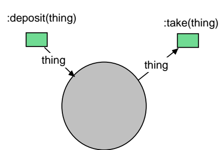
Figure 4.6: The net iconbag
